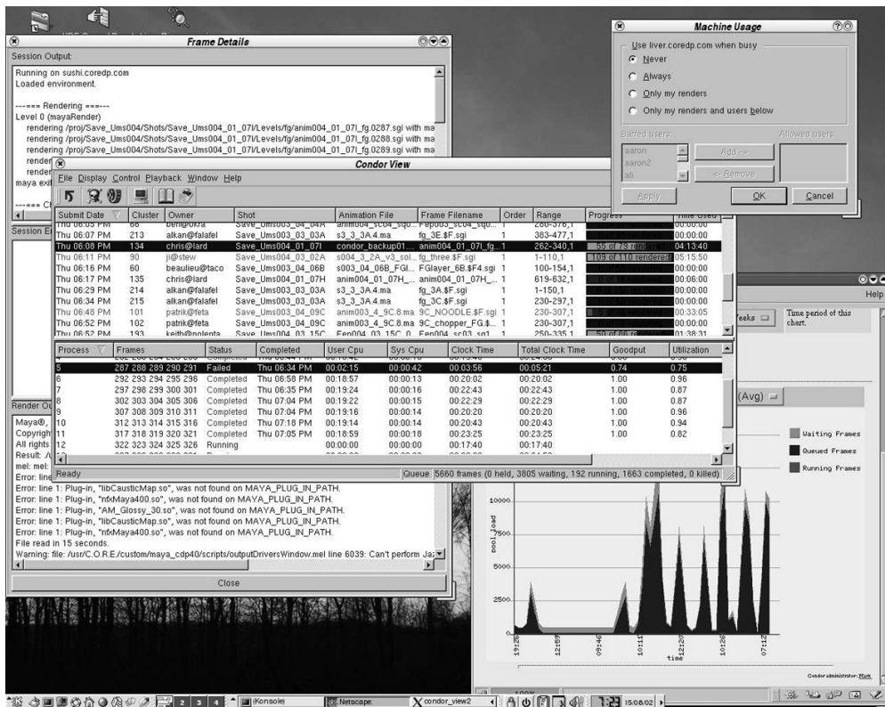
Figure 11.19 Vertical integration of Condor for computer animation. Custom GUI and database integration tools sitting on top of Condor help computer animators at C.O.R.E. Digital Pictures.
